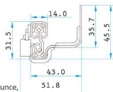
NJ-A5807 Short Drawer Frame
