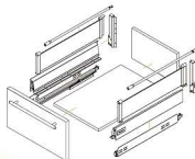
NJ-A5809 Tall Drawer Frame
