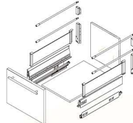
NJ-A5810 Dual Rail Drawer Frame
